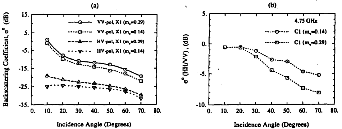
Figure 2. Angular plots of (a) \sigma_{vv}^0 and \sigma_{hv}^0 of surface S1 at X-band for two different moisture conditions and (b) the like-polarized ratio, \sigma_{hh}^0 / \sigma_{vv}^0 , for the same surface at C-band.
