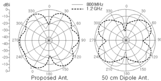
(b) 수직 방향 복사 패턴 (b) The radiation pattern along the vertical plane
