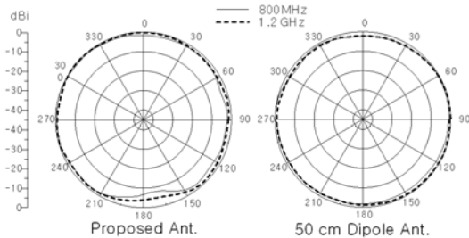
(a) 수평 방향 복사 패턴 (a) The radiation pattern along the horizontal plane
