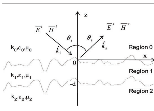
Fig. 1. Geometry of the two-layered medium.
