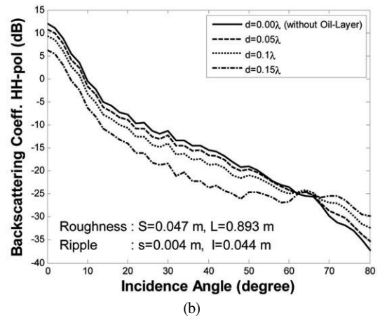
Fig. 5. Reduction of the backscattering coefficients by the oil layer for (a) VV- and (b) HH-polarizations.
